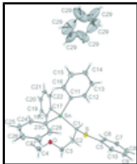
Fig. 1. Structure of the title compound. Displacement ellipsoids are drawn at the 30% probability level and the H atoms are shown as small spheres of arbitrary radii.
