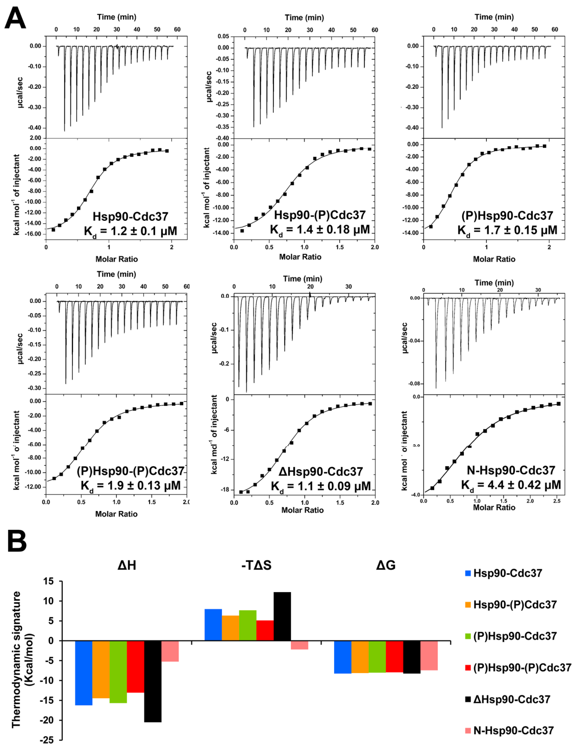
Figure 2. Influence of phosphorylation by CK2 on the thermodynamics of Hsp90 \beta -p50 Cdc37 complex formation. (A) Isothermal titration calorimetry (ITC) experiments of the Hsp90 \beta -p50 Cdc37 complex formation using unphosphorylated and phosphorylated proteins. The last two graphs show the interactions of Hsp90 without the acidic loop ( \Delta Hsp90) and of the N-terminal domain (N-Hsp90); (B) Thermodynamic signatures of the protein-protein interactions (PPI).
