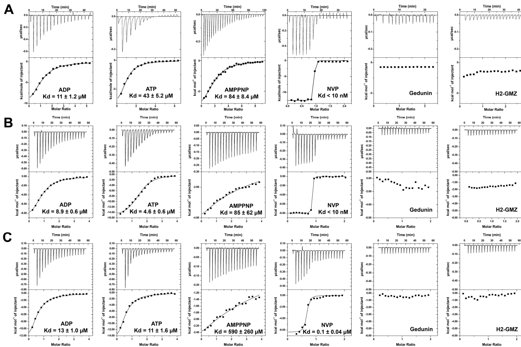
Figure 3. Interaction of Hsp90 \beta proteins with nucleotides and reported inhibitors determined by ITC. Shown are the results of titration experiments for small molecule ligands with \Delta Hsp90 \beta (A); full-length Hsp90 \beta (B); and CK2-phosphorylated Hsp90 \beta (C).
