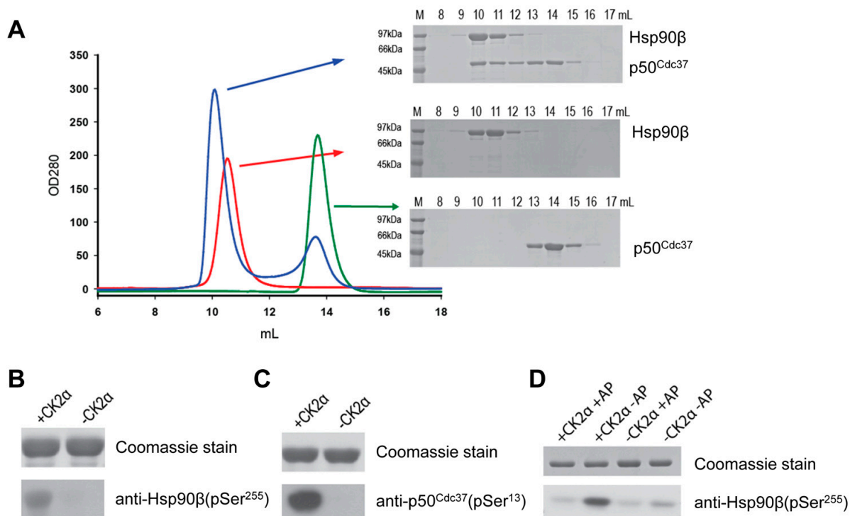
Figure 1. In vitro reconstitution of the human full-length Hsp90β:p50 Cdc37 complex and phosphorylation by CK2α. (A) Elution profiles and corresponding SDS-PAGE for analytical gel filtration experiments showing complex formation (blue) upon incubation of free Hsp90β (red) with free p50 Cdc37 (green). (B) Coomassie-stained SDS-PAGE and Western blot analysis of purified Hsp90β in the presence and absence of CK2α and ATP using anti-Hsp90β (pSer 255 ); (C) Coomassie-stained SDS-PAGE and Western blot analysis of purified p50 Cdc37 in the presence and absence of CK2α and ATP using anti-p50 Cdc37 (pSer 13 ); (D) Phosphorylation states of Ser255 in Hsp90β upon phosphorylation by CK2α and dephosphorylation by alkaline phosphatase (AP).
