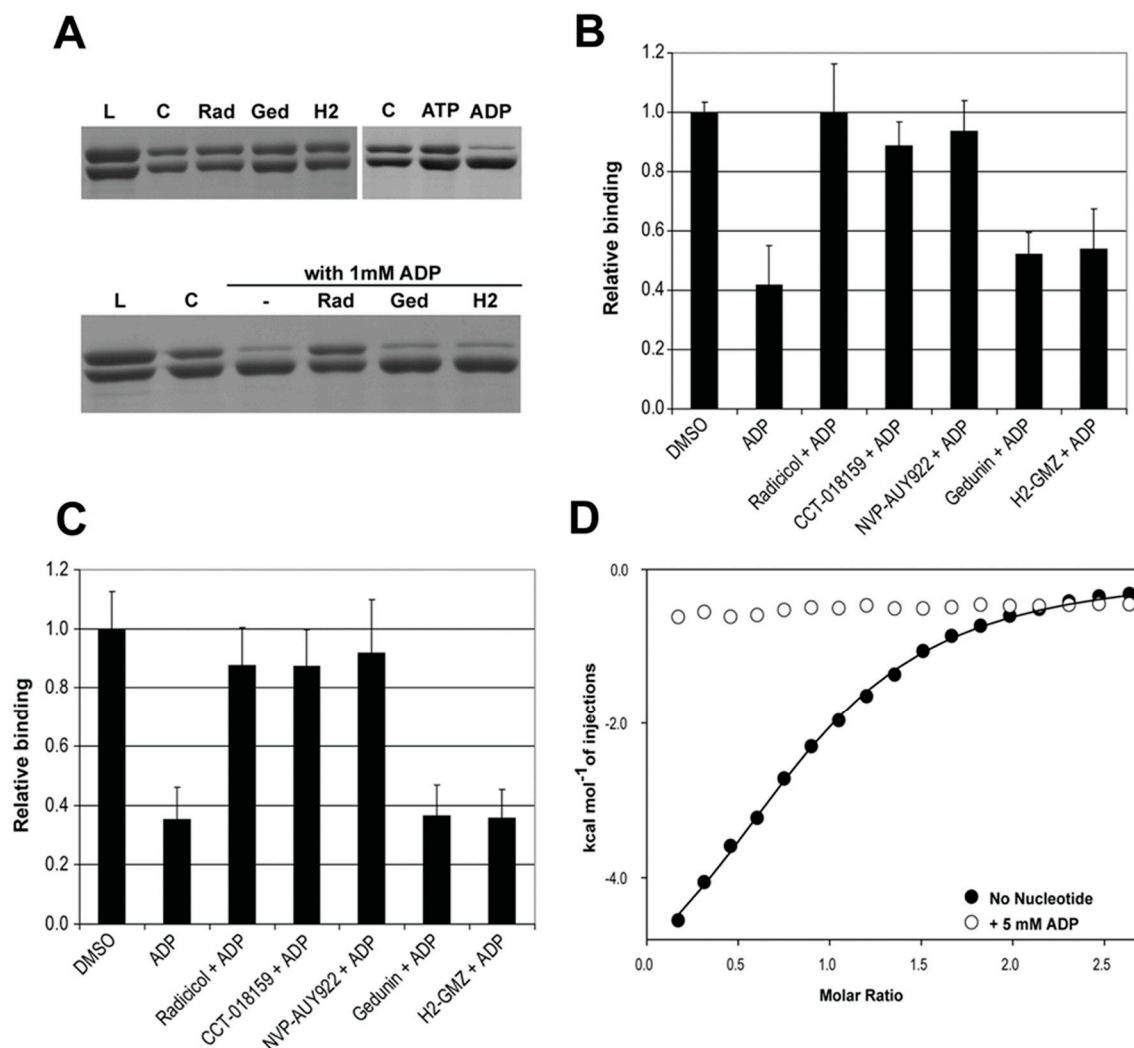
Figure 5. The PPI inhibitory activity of ADP proceeds through binding to the ATP site of Hsp90. (A) SDS-PAGE of GST pull-down experiments for \Delta\text{Hsp90}\beta interaction with GST-p50 Cdc37 . The two proteins were incubated with 1 mM nucleotide or 0.1 mM inhibitor for 15 min, loaded onto a GST-affinity column, and eluted with reduced glutathione. The upper gels show elution of a stable complex in the presence of inhibitors or ATP, but the presence of ADP caused disruption of the complex. The bottom gel shows the result of a competition experiment in which the presence of 0.1 mM radicicol protected the complex from ADP, whereas gedunin and H2-GMZ had no effect. L = load, C = control (no ligand), Rad = radicicol, Ged = gedunin, H2 = H2-GMZ; (B,C) Competition experiments for the interaction of \Delta\text{Hsp90}\beta (B) or \Delta\text{Hsp90}\alpha (C) with p50 Cdc37 in the presence of 1 mM ADP and 0.25 mM inhibitors (0.1 mM for gedunin) determined by ELISA. Only ATP site-directed inhibitors protected the complex from ADP; (D) Binding isotherms for the interaction of the N-terminal domain of Hsp90 \beta with p50 Cdc37 in the absence and presence of ADP.
