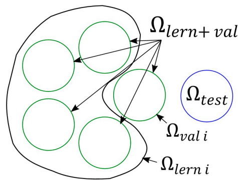
Figure 3. Data division.
