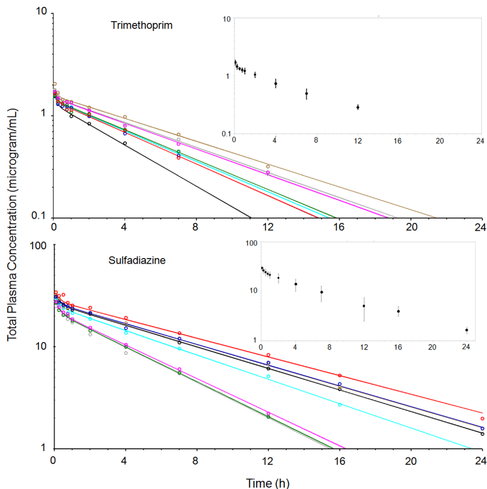
FIGURE 1 Spaghetti plot of observed (circles) and model predicted (lines) trimethoprim total concentration-time courses (upper plot) and sulfadiazine total concentration-time courses (lower plot) following the last of five intravenous 2.5 mg/kg trimethoprim and 12.5 mg/kg sulfadiazine administrations every 12 h to eight neonatal foals. The trimethoprim/sulfadiazine combination was administered at -48, -36, -24, -12 and 0 h. Insets show mean \pm SD observed total trimethoprim and sulfadiazine concentrations
