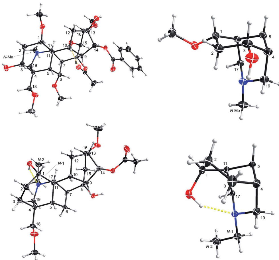
Fig. 3 SXR D data of mesaconitine (5, upper) and condelphine (7, lower), and their A/E-[3.3.1]azabicyclic frames. ORTEP presentations of the crystal structures show the atom position with a 50% probability for each ellipsoid.
