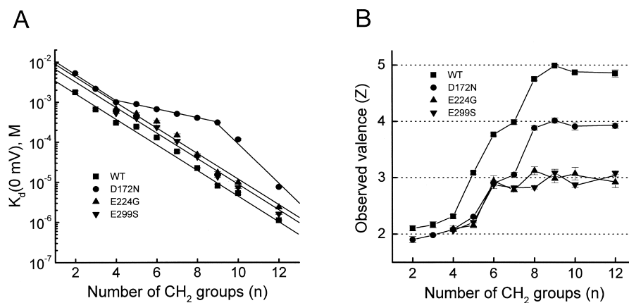
FIGURE 12. Summary of dissociation constants and valences for steady-state channel block by alkyl-bis-amines. Shown in A and B are values of K_d(0 \text{ mV}) and Z , respectively (mean \pm SEM; n = 4-6 ), determined from fits as shown in Fig. 11), for block of wild-type and three single mutant channels by a series of bis-amines of varying chain length. Bis-C11 is not available commercially.
