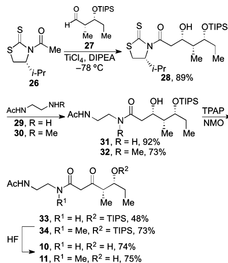
Scheme 1. Synthesis of Amide Substrate Analogs 10 and 11
