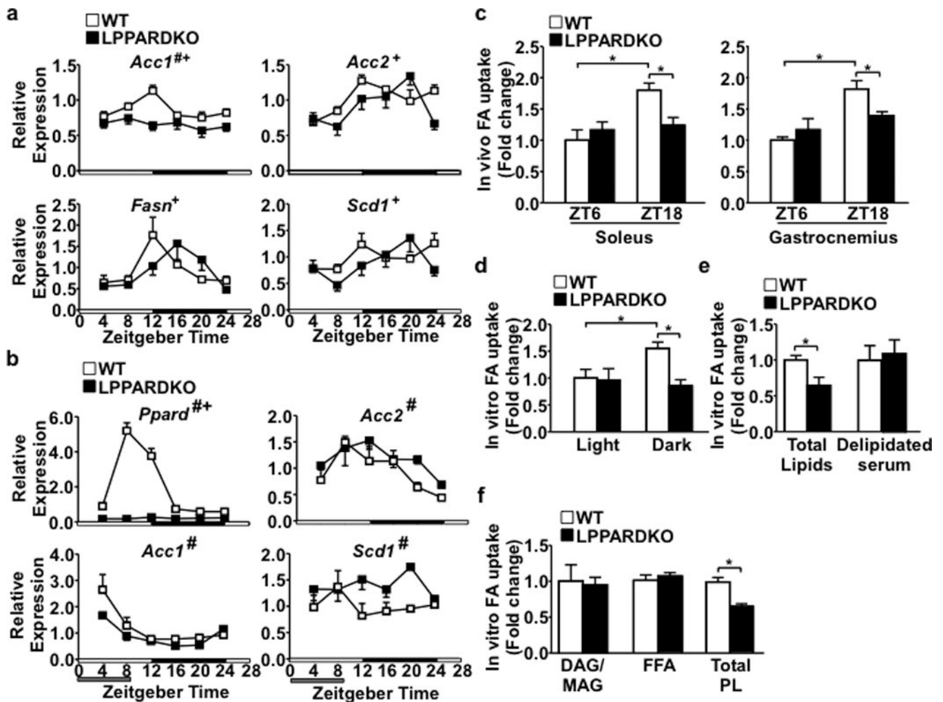
Figure 2. Hepatic PPAR \delta controls liver lipogenic gene expression and muscle FA uptake a. Hepatic lipogenic gene expression in wt and LPPARDKO mice ( n=4/\text{time point} ). White and black bars on the x-axis represent light and dark cycles, respectively. b. Liver gene expression under daytime feeding ( n=3 ). # p<0.05 (ANOVA), wt vs. LPPARDKO; + p<0.05 , comparing circadian patterns. c. In vivo muscle fatty acid uptake ( n=3 ). d.-f. In vitro fatty acid uptake in C2C12 myotubes treated with serum (2%) pooled from light or dark cycle samples, serum total lipids or delipidated serum (dark cycle samples) or serum lipid fractions ( n=3 ). * p<0.05 (t-test), data shown as mean \pm SEM.
