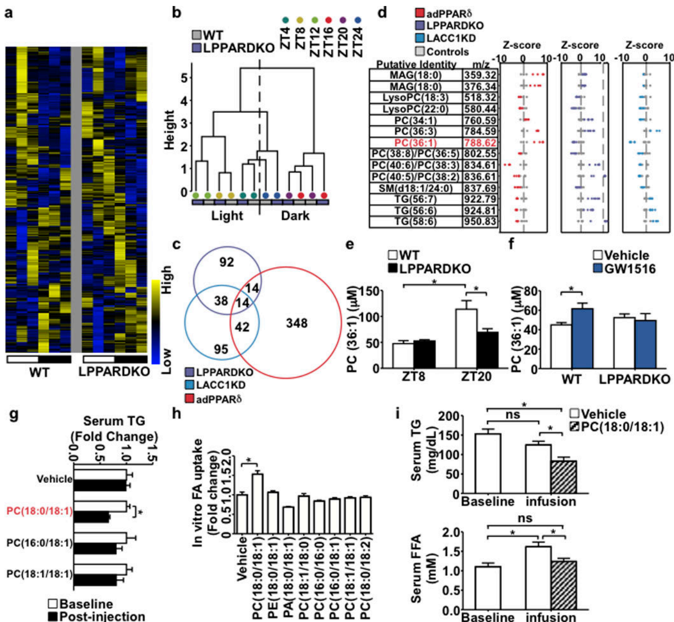
Figure 3. PC(18:0/18:1) links hepatic PPAR \delta to serum lipid levels and muscle FA uptake a. Serum lipid heatmap (n=3/time point). White = light (starting at ZT4) and black = dark cycles. b. Dendrogram from hierarchical clustering. c. Cross-comparison of changed lipids. d. Z-score plots of 14 commonly changed features. e. Serum PC(36:1) quantification in wt (n=5) and LPPARDKO (n=4) mice. f. Serum PC(36:1) concentrations in wt/LPPARDKO \pm GW501516 (n=5). g. Serum TG changes (tail vein injection) with PLs in wt mice (n=6). h. FA uptake in C2C12 myotubes treated with PLs (50 \mu M, n=3). i. Serum TG and FFA levels after PC(18:0/18:1) infusion (n=6, wt C57BL/6J mice). *p<0.05 (t-test), data presented as mean \pm SEM.
