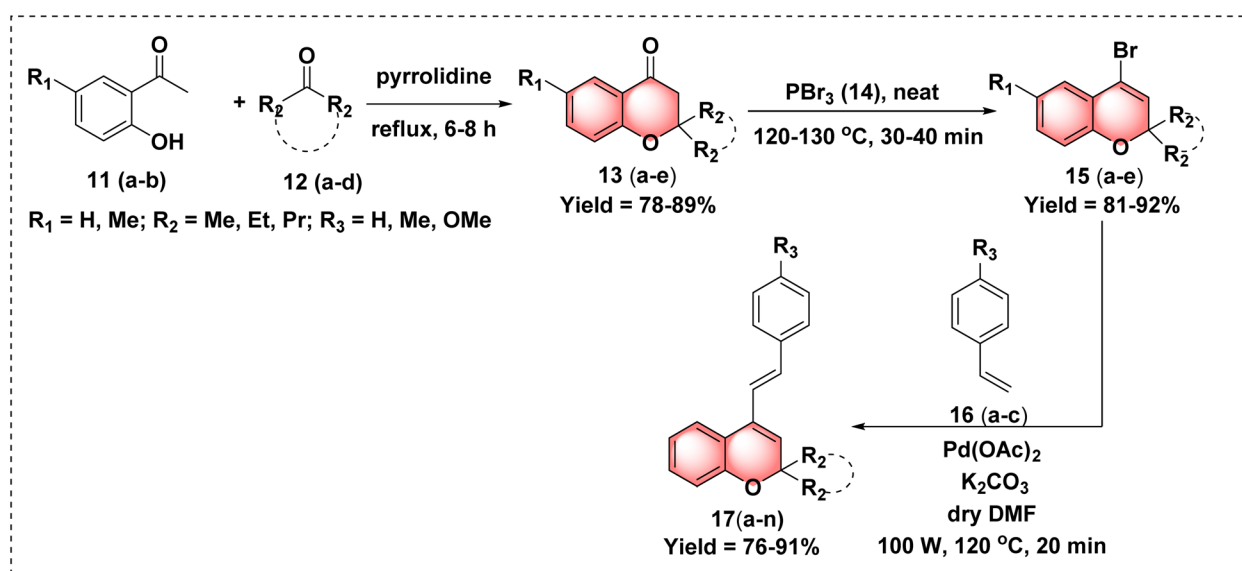
Scheme 1 Synthesis of 2,2-disubstituted chromenes 13(a-e), 4-bromo-2,2-dialkylsubstituted-2H-chromenes 15(a-e) and 2,2-disubstituted-4-styryl-2H-chromene 17(a-n).
