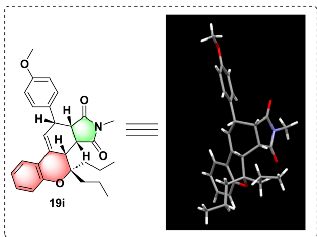
Fig. 3 Single crystal X-ray representation of compound 19i .
