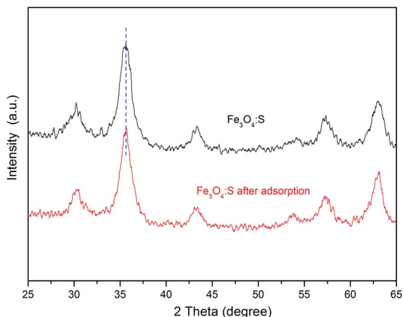
Fig. 7 XRD spectra of Fe 3 O 4 :S NPs before and after As(v) adsorption. Experimental conditions: initial As(v) concentration was 50 mg L -1 (100 mL), adsorbent dosage was 60 mg, pH 6, contact time was 24 h, temperature was 30 °C.
