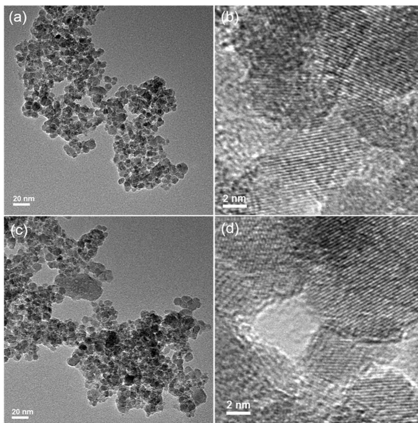
Fig. 8 TEM images of Fe 3 O 4 :S NPs before and after As(v) adsorption. (a and b) TEM and the corresponding HR-TEM image of Fe 3 O 4 :S NPs; (c and d) TEM image and the corresponding HR-TEM image of Fe 3 O 4 :S NPs after adsorption. Experimental conditions were the same as above.
