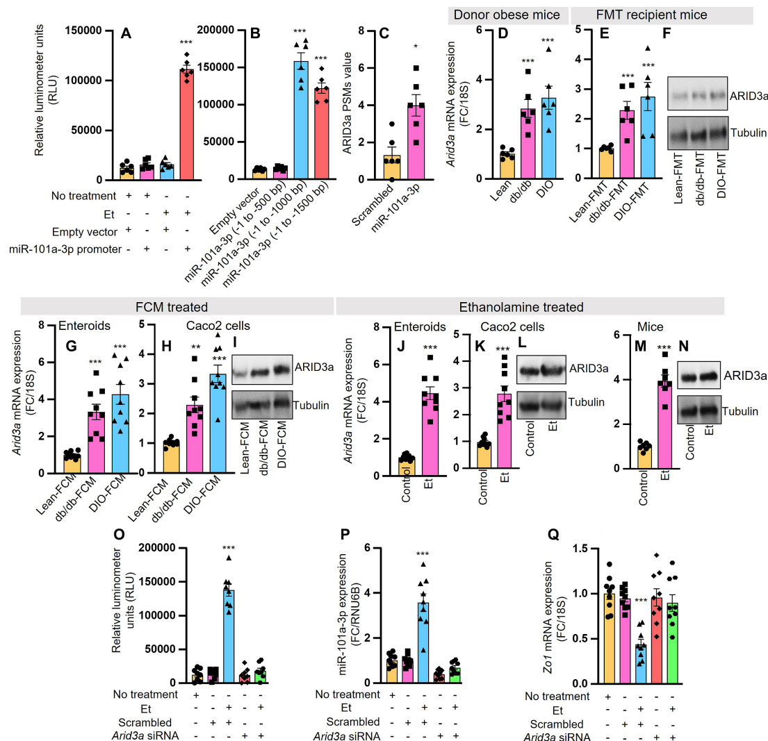
Figure 5 Ethanolamine increases miR-101a-3p expression by increasing its promoter activity by enhancing transcription factor ARID3a binding on it. (A) Ethanolamine increased miR-101a-3p promoter depicted by luciferase assay in Caco-2 cells transfected with a vector carrying miR-101a-3p promoter (–1 to –2000 bp of transcript start site (TSS)) compared with empty vector-transfected cells. (B) Further, ethanolamine treatment significantly increased miR-101a-3p promoter activity in the Caco-2 cells transfected with vectors carrying –1 to –1000 bp and –1 to 1500 bp fragments, while no change was observed in cells transfected with a vector carrying –1 to 500 bp and empty vector. (C) Unbiased and untargeted ChIP- pull-down analyses revealed that a transcription factor-ARID3a was the highest protein pulled out with –500–1000 bp fragment compared with a scrambled nucleotide DNA sequence. (D, E) Interestingly, expression of Arid3a mRNA (D, E) and protein (F) was found significantly higher in the gut of donor db/db and DIO mice (D) as well as in FMT recipients (E, F) (G–I) In addition, obese/T2D FCMs (G–I) and ethanolamine (J–N) treatments significantly increased the expression of Arid3a in the enteroids (G, J), Caco-2 cells (H, I, K, L) and mouse intestine (M, N) compared with controls. (O–Q) Notably, ethanolamine-mediated activation of miR-101a-3p promoter activity (O), miR-101a-3p expression (P), and suppression in Zo1 expression (Q) were abolished in ARID3a siRNA transfected Caco-2 cells compared with scrambled siRNA transfected cells. Values presented are the mean of n=5-8 mice, n=2-3 repeated triplicate enteroids and Caco-2 culture experiments in each group; error bars are the SEM. * p<0.05 , ** p<0.01 , *** p<0.001 are statistically significant analysed by independent t-test and/or ANOVA. ANOVA, analysis of variance; FCM, faecal conditioned media; FMT, faecal microbiota transplantation; T2D, type 2 diabetes.
