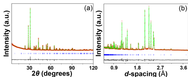
Fig. 4 Rietveld refinement plots of (a) XRD data and (b) ND data for the Ba 4 SbMn 3 O 12 sample, showing observed (red crosses), calculated (green line), and difference curve (grey line). The reflection positions for Ba 4 SbMn 3 O 12 are marked with blue bars in both plots.
