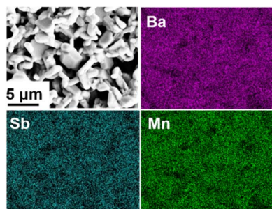
Fig. 3 SEM image and EDS elemental mapping image on the Ba 4 SbMn 3 O 12 sample, indicating the homogeneous distribution of elements.
