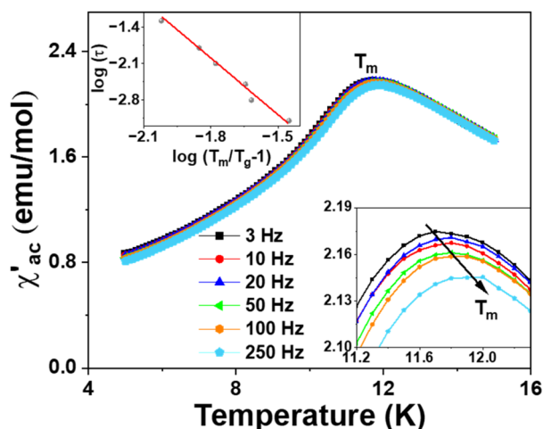
Fig. 8 Temperature dependence of the real ac susceptibility component \chi'_{ac} at frequencies of 3 \leq f \leq 250 Hz. The bottom inset shows the data around T_m for clarity. The top inset shows the frequency dependence of the freezing temperature T_m with the best power-law fit.
