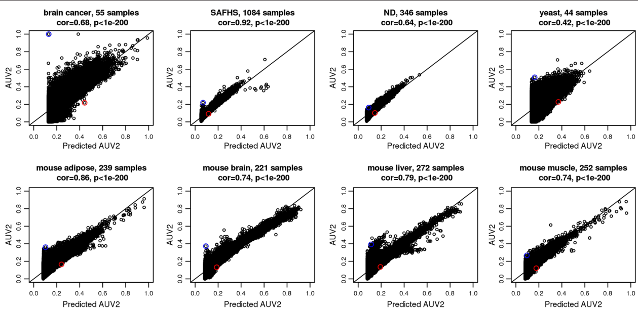
Figure 3 Comparison of predicted and observed A^{MI, UniversalVersion2} in 8 empirical data sets. In all data sets, prediction from bicor based on Eq. 18 and observed A^{MI, UniversalVersion2} are highly correlated (the Pearson correlation and corresponding p-value shown at top). Line y=x is added. Blue and red circles have the same meaning as in Figure 2.
