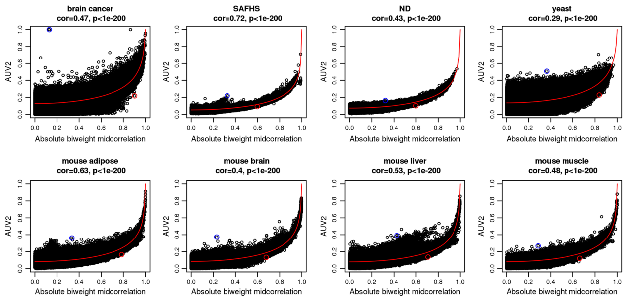
Figure 2 Comparison of correlation and mutual information based co-expression measures in 8 empirical data sets. Absolute value of bicor versus A^{MI, UniversalVersion2} for all probe pairs in each data set. The Spearman correlation and corresponding p-value between the two measures are shown at the top. The two measures show different levels of monotonic relationships in data sets. The red curve predicts A^{MI, UniversalVersion2} from bicor based on Eq. 18. The blue circle highlights the probe pair with the highest A^{MI, UniversalVersion2} z-score among those with insignificant bicor z-scores (less than 1.9); the red circle highlights the probe pair with the highest bicor z-score among those with insignificant A^{MI, UniversalVersion2} z-scores (less than 1.9).
