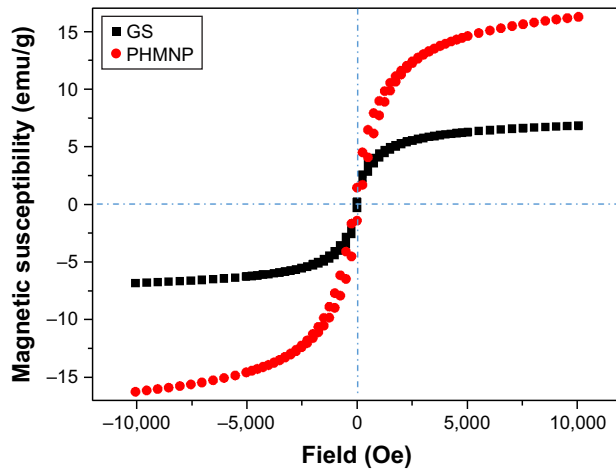
Figure S4 SQUID curves of GSs and PHMNPs.
