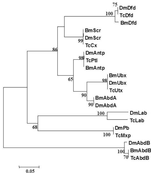
Fig. 2 Protein-sequence-based analysis of the evolutionary relatedness of various homeodomains. Panels depict Hox gene phylogenies for Tribolium , Bombyx and Drosophila . A combined tree of all the available members of classical Hox proteins from these three insect taxa was constructed by Neighbour-joining method as implemented in MEGA3 software (19), with bootstrap analysis. The sequences used were derived by translating the data from sequences listed in Table 1. The Tribolium Hox homologues have been depicted with their classical nomenclature. m xp ( maxillapedia ): pb homologue; Cx ( Cephalothorax ): Scr homologue; ptl ( prothoraxless ): Antp homologue; Utx ( Ultrathorax ): Ultrathorax homologue; and A ( Abdominal ): abdA homologue. The scale bar indicates the distance between different sequences. The bootstrap values of various nodes are marked. The nodes with no value displayed had low support values (below 70). All the nodes represented a bootstrap support value above 50. The scale bar indicates the distance between various sequences. Note the grouping of AbdB with pb and lab group of anterior genes.
