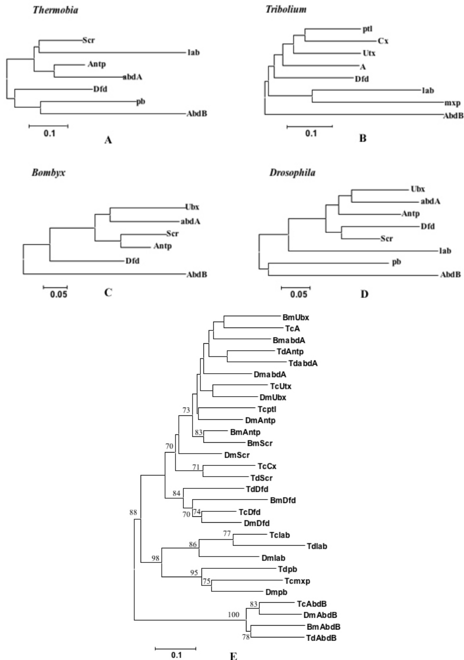
Fig. 1 Evolutionary relatedness of various members of Hox cluster. A–D. Phylogenetic analysis of Hox cluster from four representative insect taxa. Panels depict Hox gene phylogenies for Thermobia (A), Tribolium (B), Bombyx (C), and Drosophila (D). The phylogenetic trees were constructed by Neighbour-joining method as implemented in MEGA2 software (17), with bootstrap analysis. All the nodes represented a bootstrap support value above 50. The sequences used and their GenBank accession numbers are listed in Table 1. The Tribolium Hox homologues have been depicted with their classical nomenclature. mxp ( maxillapedia ): pb homologue; Cx ( Cephalothorax ): Scr homologue; ptl ( prothoraxless ): Antp homologue; Utx ( Ultrathorax ): Ultrabithorax homologue; and A ( Abdominal ): abdA homologue. The scale bar indicates the distance between different sequences. E. A combined tree of all the available members of Hox clusters from the four insect taxa was constructed using the Neighbour-joining method as implemented in the MEGA3 software (19) with bootstrap analysis. The bootstrap values of various nodes are marked. The nodes with no value displayed had low support values (below 70). The scale bar indicates the distance between various sequences. Note the grouping of AbdB with pb and lab group of anterior genes.
