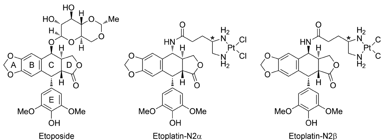
Figure 1. Chemical structures of etoposide and the two etoplatis synthesized in this study. The polycyclic aglycone (rings A–D) and pendant ring (E-ring) of etoposide are labeled. A cis -dichlorodiammineplatinum(II) moiety was introduced via an amide linkage to the C4 position of the aglycone core in \alpha and \beta configuration about the E-ring to produce etoplatin-N2 \alpha and N2 \beta , respectively. Both etoplatis contain an additional chiral center (marked with asterisks) whose chirality was not specified during synthesis.
