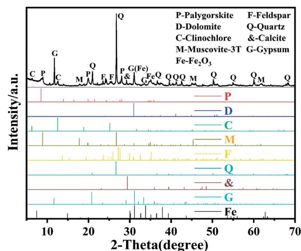
Fig. 1 XRD pattern of raw palygorskite clay.
