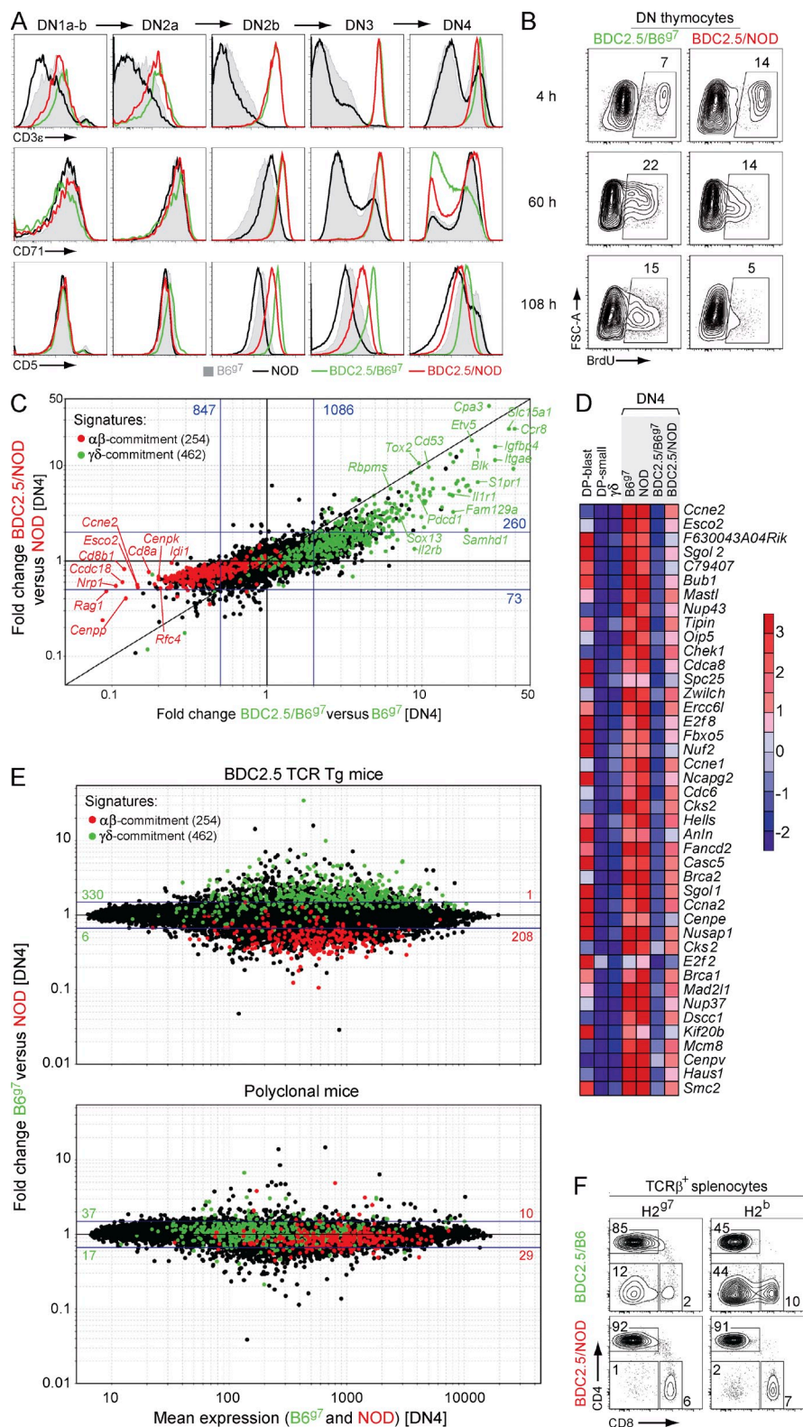
Figure 7. B6 and NOD \alpha\beta -TCRs promote opposite \gamma\delta^- and \alpha\beta -lineage fates. DN thymocytes (A–E) or splenocytes (F) were isolated from non-tg or BDC2.5 TCR tg mice. (A) Expression of CD3e, CD71, and CD5 on DN subsets (defined as shown in Fig. S4 A). (B) BrdU pulse-labeling experiment. Density plots show intracellular levels of incorporated BrdU in DN thymocytes at different times after a single BrdU injection. (C) Fold change/fold change plot depicting the BDC2.5 tg/non-tg ratio of expression in B6 97 (x axis) and NOD (y axis) DN4 thymocytes. Blue lines, fold change of 2 (with the number of genes in the corresponding areas). (D) Heat map of 42 cell cycle-related transcripts down-modulated in BDC2.5/B6 97 DN4 thymocytes (relative expression is color-coded). Cycling (blast) and noncycling (small) DP and \gamma\delta thymocytes from ImmGen datasets are included for comparison. (E) Fold change versus mean expression plot depicting B6 97 versus NOD DN4 thymocyte subsets from BDC2.5 TCR tg (top) and polyclonal mice (bottom). Blue lines, fold change of 1.5. The number of \gamma\delta and \alpha\beta signature genes above and below this threshold is indicated in green and red, respectively. (F) Proportion of \gamma\delta -like CD4 - CD8 - DNs on gated TCR- \beta^+ splenocytes from mice of indicated genotypes. Mean frequencies: 15.4 \pm 4.9 (BDC2.5/B6 97 ) versus 0.6 \pm 0.2 (BDC2.5/NOD); 32.1 \pm 11.3 (BDC2.5/B6) versus 3.8 \pm 1.5 (BDC2.5/NOD.H2 b ). Data are representative of three (A; n \geq 9 per genotype), eight (B; n \geq 25 per genotype), two (C–E; n = 2 per genotype per experiment), and three (F; n \geq 10 per genotype) independent experiments.
