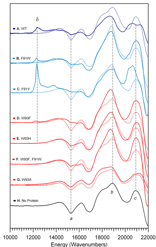
Figure 7. MCD spectra at 4.5 K and 7 T of Co(II)Cbl obtained in the presence of \text{SeCobA}^{\text{WT}} and various variants. Solid lines show the spectra in the presence of ATP, while dotted lines are the corresponding traces in the absence of ATP. Panels A–G are labeled according to the amino acid substitution(s) introduced into \text{SeCobA} . The feature due to 4c Co(II)Cbl species (band \delta ) is highlighted by a vertical line. The relevant MCD features of free Co(II)Cbl (H) are labeled with lowercase Latin letters, and their positions are also highlighted by vertical lines.
