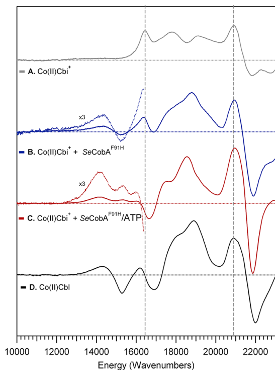
Figure 9. MCD spectra collected at 4.5 K and 7 T of (A) free Co(II)Cbi + , (B) Co(II)Cbi + in the presence of SeCobA, and (C) Co(II)Cbi + in the presence of SeCobA and ATP. For reference, the spectrum of free Co(II)Cbl is shown in panel D. The most intense features of free Co(II)Cbi + are highlighted by dashed vertical lines. The lower-energy region of the spectra of protein-bound species is scaled by a factor of 3 to highlight unique features in this region.
