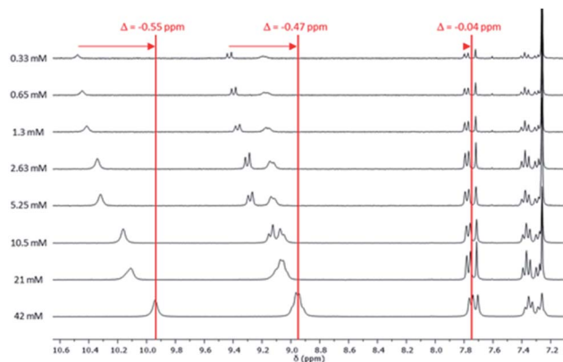
Fig. 3 ^1\text{H} NMR spectra of reference 6 at different concentrations (0.33–42 mM) between 7.1 and 10.5 ppm (phenyl aromatic region) in \text{CDCl}_3 at 25 °C.
