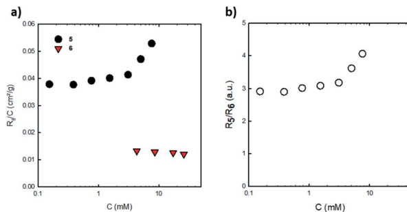
Fig. 5 (a) Rayleigh ratios normalized by concentration for solutions of penta(BPTI)[60]fullerene 5 and reference 6 in \text{CHCl}_3 at 20 °C. (b) Ratio of Rayleigh ratios of 5 and 6 against 5 concentration.
