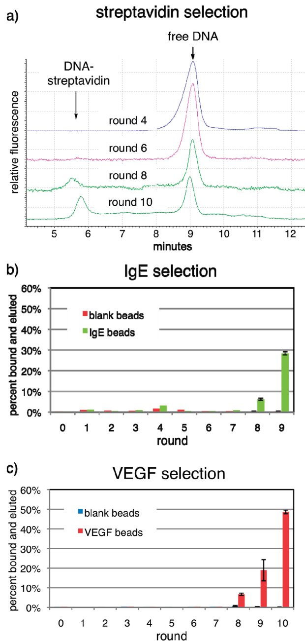
Figure 2. Binding activity of pools over 9 to 10 rounds of selections for binding (a) streptavidin, (b) IgE, and (c) VEGF.
