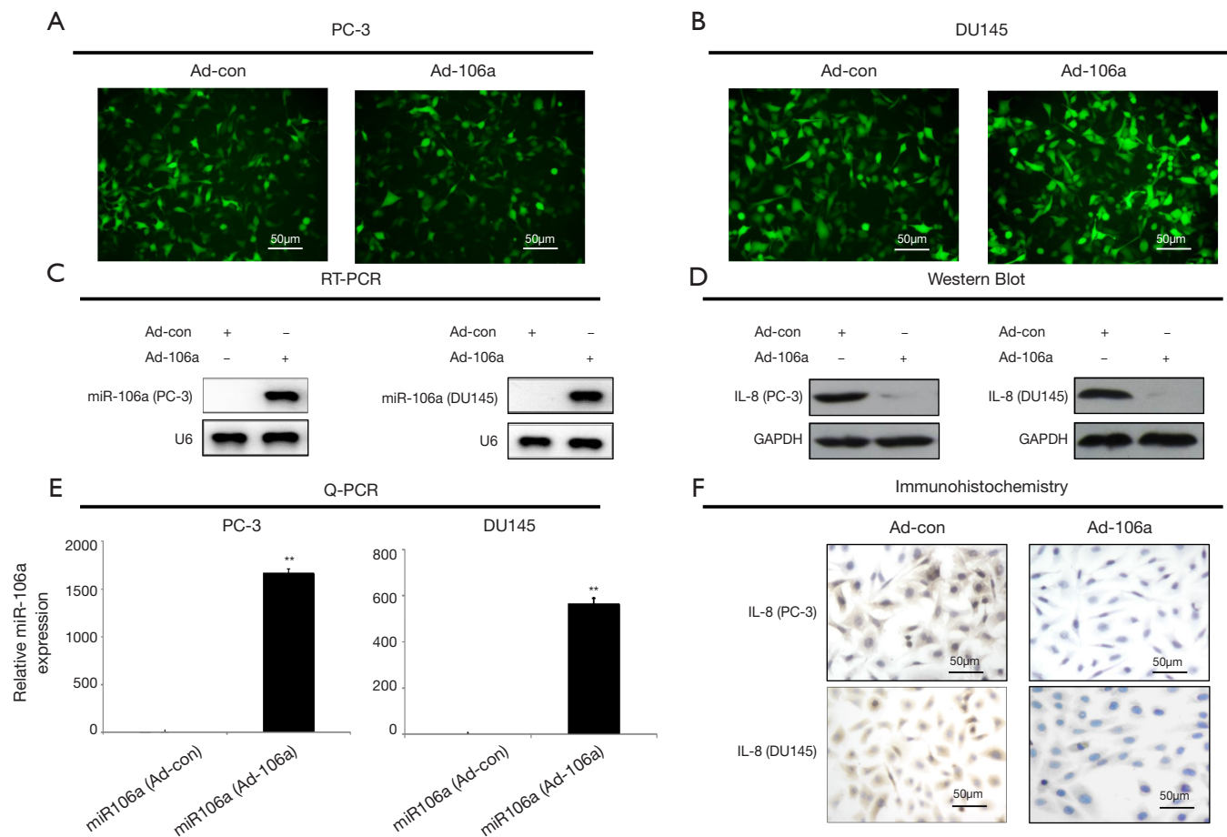
Figure 2 The effects of artificial miR-106a over-expression on IL-8 in PC-3 and DU145 cells. Homogenous green fluorescence protein expression (A,B), RT-PCR (C) and Q-PCR (E) demonstrated the differential expression of miR-106a expression following infected with Ad-miR-106a or Ad-control in PC-3 and DU145 cells. Western blot analysis (D) and immunocytochemistry (F) showed the changes in IL-8 protein levels following transfected with Ad-miR-106a or Ad-control in PC-3 and DU145 cells. The bar within the picture, 50 \mu m. Double asterisks indicate P < 0.001 .
