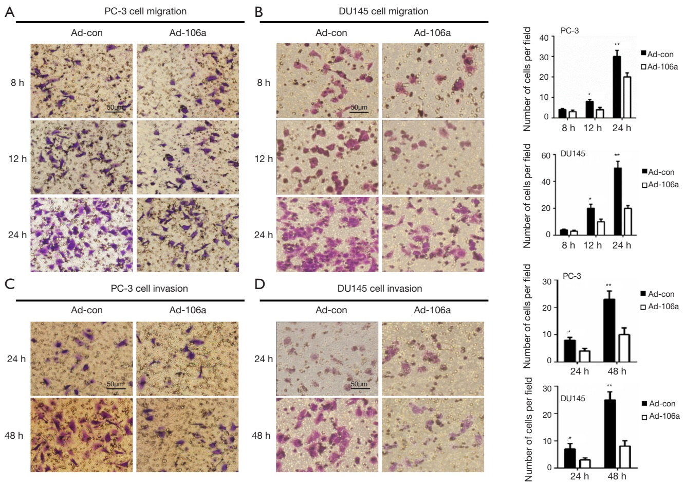
Figure 5 The effects of miR-106a overexpression on migration and invasion in the transwell culture system. The migration function of PC-3 (A) and DU145 (B) (compared to Ad-con) cells was significantly inhibited after miR-106a overexpression. The invasion capability of PC-3 (C) and DU145 (D) (compared to Ad-con) cells was significantly restrained following miR-106a overexpression. Cells were stained by methylrosanilium chloride solution. The bar within the picture. A single asterisk indicates P < 0.05 . Double asterisks indicate P < 0.001 .
