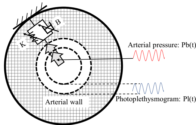
Figure 1. Schematic diagram of the mechanical impedance model. The model used in this study consists of a parallel arrangement of springs and dampers across the diameter of the arterial wall. When a force (blood pressure) is applied across the diameter of the artery, the arterial wall is damped by springs and dampers that represent the rigidity and viscosity of the arterial wall itself. The behavior of the arterial wall after damping is observed as a change in the photoplethysmogram waveform.
