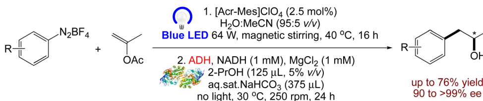
Scheme 10 Synthesis of enantiopure 1-arylpropane-2-ols from aryl diazonium salts via a photobiocatalytic cascade. 84
