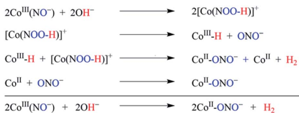
Scheme 3 NOM reaction of complex 1 in the presence of \text{OH}^- , showing the different steps of the reaction.
