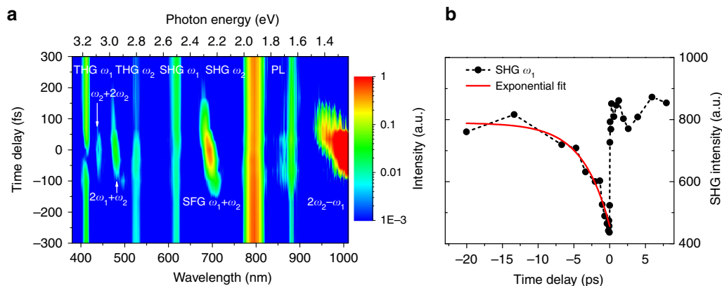
Fig. 3 Temporal dynamics of nonlinear frequency mixing. a 2D contour image of the transient nonlinear signal (logarithmic scale) when the time delay between the two pump pulses is varied. The nonlinear signals that require only one of the pumps do not depend on the delay, while the mixing signals that rely on both pumps occur only when the two pumps overlap in time. b The quenching and the recovery of the \omega_1 SHG intensity due to the arrival of the second pump \omega_2 at the metamixer. The black dots are experimentally measured SHG intensities and the red curve is a single component exponential fit with time constant of \sim 3.7 \text{ ps}
