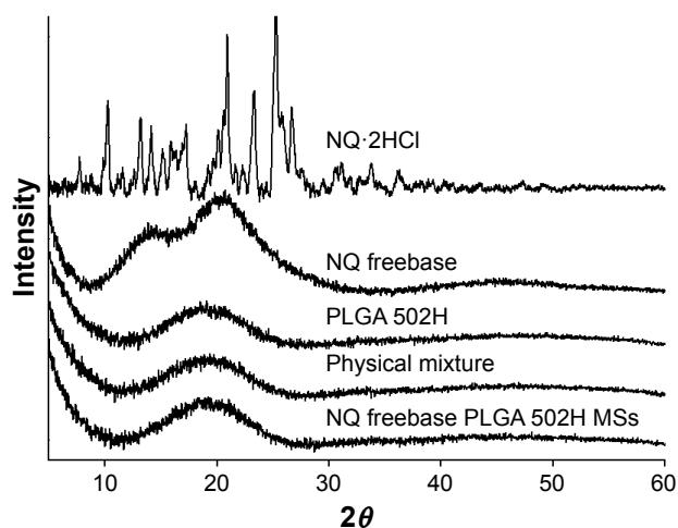
Figure 3 PXRD patterns of NQ freebase PLGA 502H MSs.
