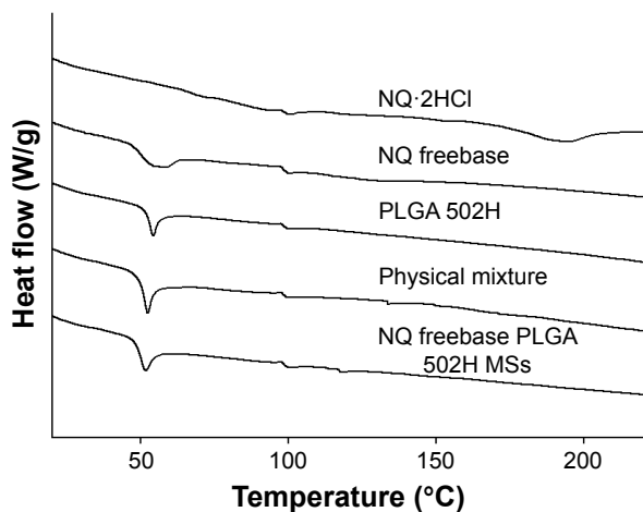
Figure 2 DSC thermograms of NQ freebase PLGA 502H MSs.
