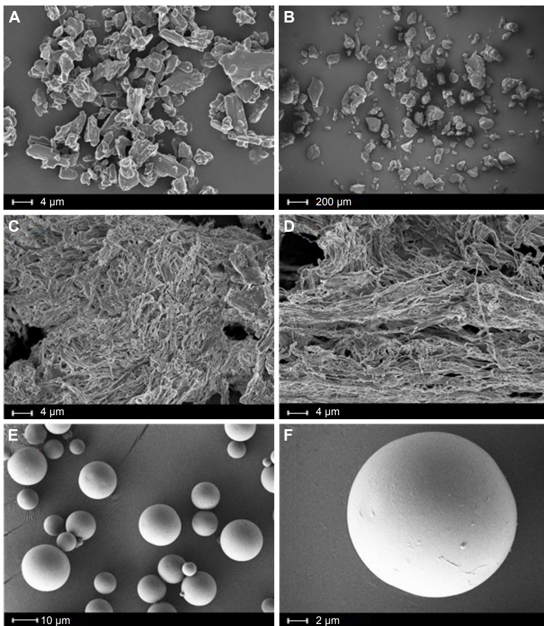
Figure 1 SEM micrographs of NQ freebase PLGA 502H MSs: (A) NQ-2HCl (5,000 \times ), (B) NQ freebase (100 \times ), (C) PLGA 502 (5,000 \times ), (D) PLGA 502H (5,000 \times ), and (E and F) NQ freebase PLGA 502H MSs (2,500 \times and 10,000 \times respectively).
