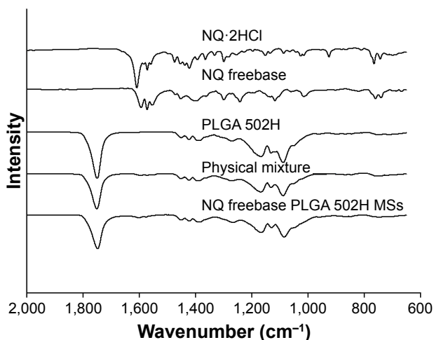
Figure 4 FT-IR spectra of NQ freebase PLGA 502H MSs.
