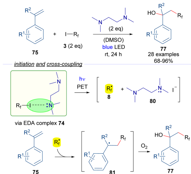
Scheme 12 Hydroxy perfluoroalkylation reaction of alkenes promoted by TMEDA.
