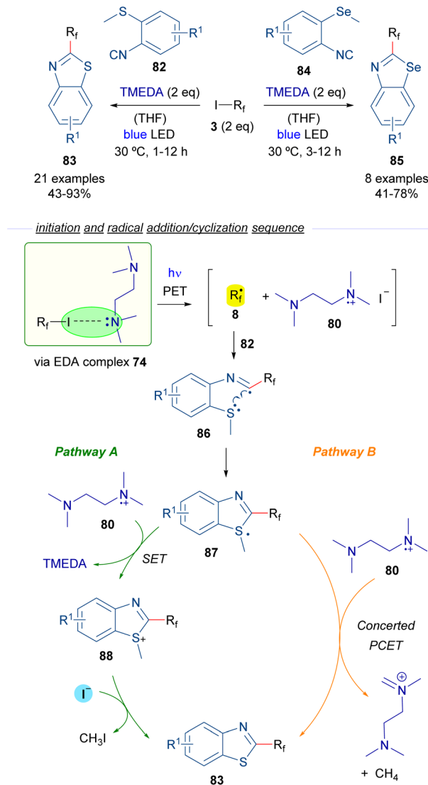
Scheme 13 Photochemical HB assisted synthesis of 2-perfluoroalkylbenzothiazoles/benzoselenazoles.
