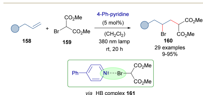
Scheme 25 ATRA reaction of olefins with bromomalonates 159 through the formation of a HB complex 161 and catalytic amounts of 4-phenylpyridine.
