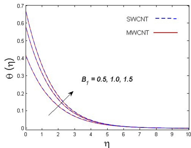
Figure 8. Outcome of B_1 on \theta(\eta) .
