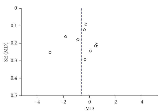
FIGURE 24: The publication bias funnel chart of TC.
