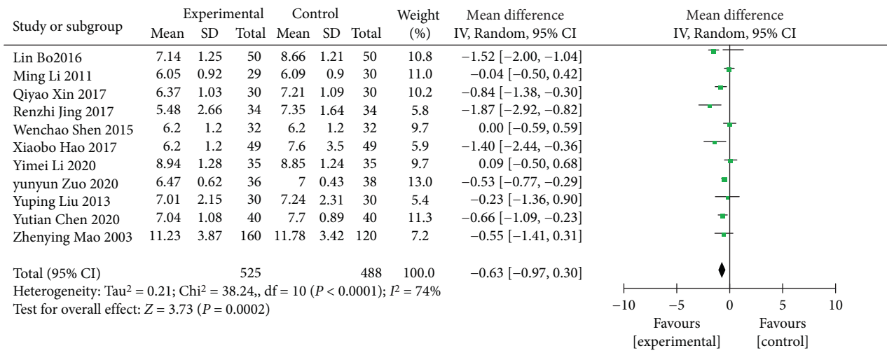
FIGURE 10: Forest plot of FBG.
