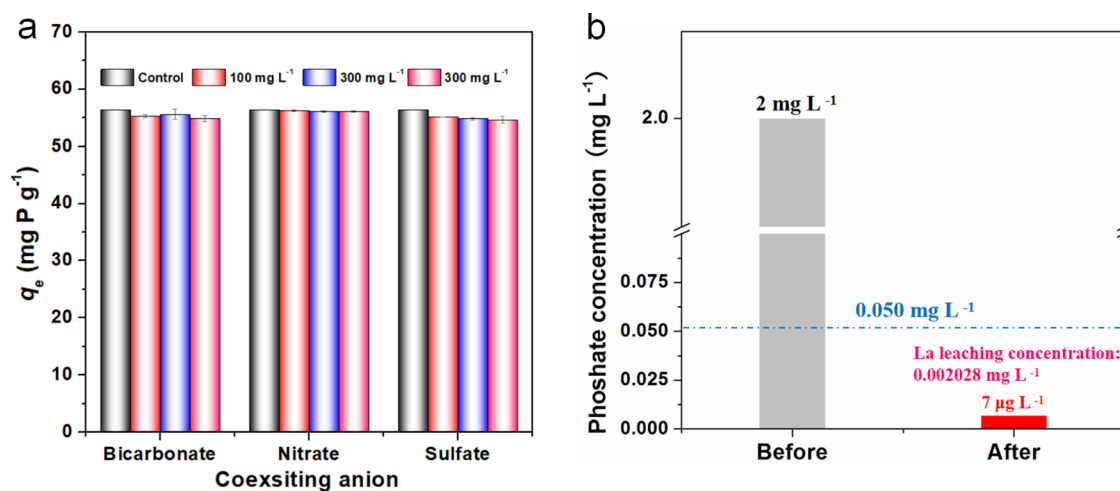
Figure 8. (a) Effect of coexisting anions on the adsorption capacity of SCBC-La for phosphate adsorption and (b) changes in the concentrations of phosphate in solution before and after 2 h treatment by SCBC-La.
