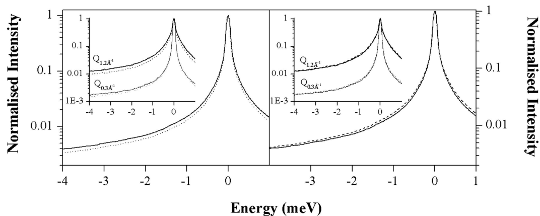
Figure 1. Quasi-elastic neutron scattering intensities, at 298 K, binned over the whole wave-vector range accessible on the IN5 spectrometer ( 0.2\text{--}2\text{Å}^{-1} ) and normalized to unity. Left panel: H30S-3 M NaCl (solid line) and H50S-3 M NaCl (dotted line), Right panel: - H30S-3 M NaCl (solid line) and H30S-3 M KCl (dashed line). Insets: same spectra at reference Q=0.3\text{Å}^{-1} (fluctuation amplitudes > 20\text{Å} ) and Q=1.2\text{Å}^{-1} (amplitudes \sim 5\text{Å} ). A broader intensity distribution indicates scattering from faster motions (see text).
