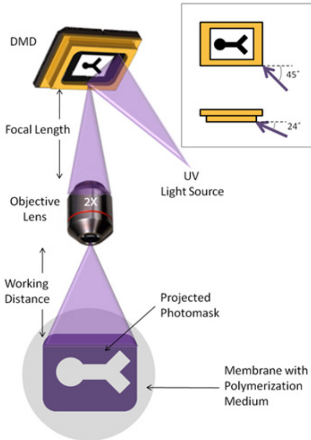
Figure 1. Schematic illustration of the light path used for photolithography. Inset: The UV light illuminates the DMD at an angle of 45°, and 24° below the plane of the mirror array.
