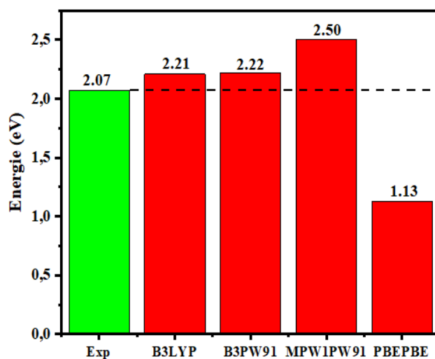
Fig. 2 E_{\text{gap}} of D1 determined using DFT with different functionals and comparison with the experimental values.
