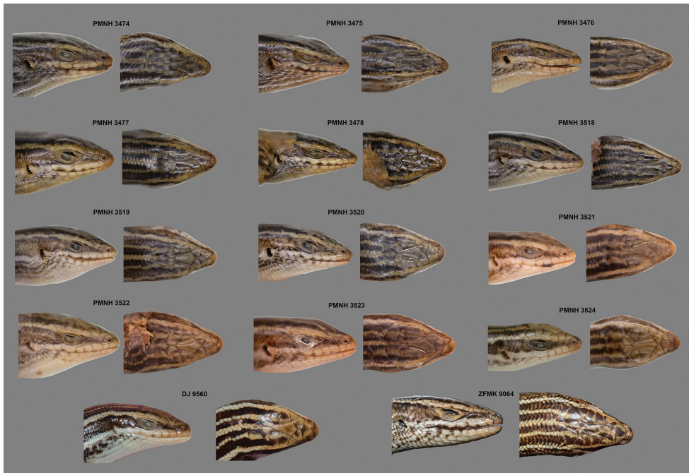
Figure 5. Lateral and dorsal head views of collected specimens of Heremites septemtaeniatus transcausicus from Pakistan (PMNH 3474–3478, PMNH 3518–3524 and DJ 9560), together with the only specimen of the species from Afghanistan (Dar-e-Nur, vic. Shewa, ZFMK-H 9064).
