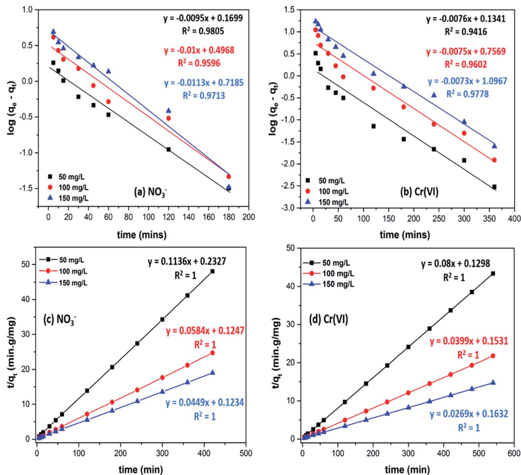
Fig. 6 Evolution in time of \log(q_e - q_t) and t/q_t for the pseudo-first order and pseudo-second order kinetics of \text{NO}_3^- (a and c) and \text{Cr}(\text{VI}) (b and d) ions adsorption onto CS-T-PEI-P ( m_{\text{ads}} = 0.2 g, initial pH, 300 rpm, V = 50 mL and 23^\circ\text{C} ).
