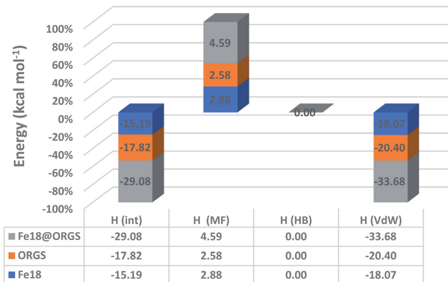
Fig. 9 ORGS@ \text{Fe}_{18} interaction energies.
