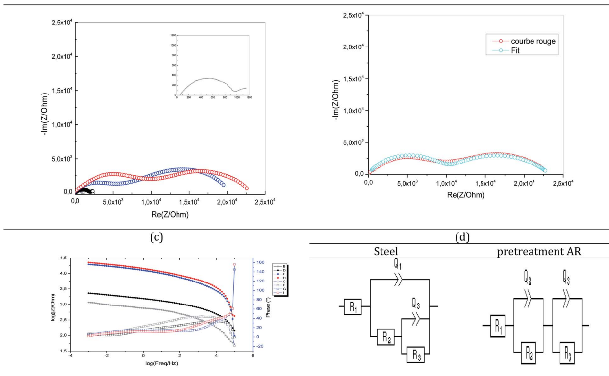
Fig. 7 (a) Experimental and (b) fitting EIS (Nyquist) of XC38 (inset, grey) 2.5 \mu\text{m} ORGS coated (black: without pretreatment; blue: pretreated with \text{N}_2 ; red: pretreated with Ar), (c) experimental EIS (BODE) and (d) equivalent circuit proposed of XC38 (steel, and pretreated with Ar).
