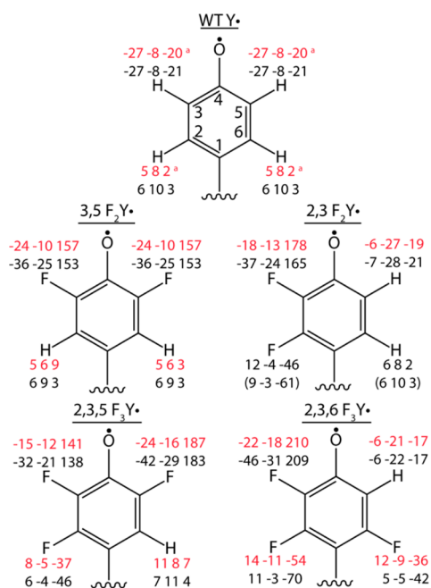
Figure 5. Hyperfine values (MHz) for ring atoms of Y_{122}\bullet and F_n Y_{122}\bullet s. Values of each component of the hyperfine tensor are presented in order as A_x , A_y , A_z . Parameters determined from simulations of the combined EPR and ENDOR data for each position are presented on top in red, and the parameters from DFT calculations are presented on the bottom in black. Experimental values for WT Y\bullet are from an ENDOR study by Hoganson et al. 84
