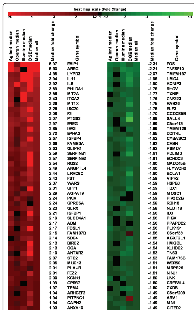
Figure 5 Top regulated genes derived from meta-analysis. RankProd analysis of the combination of microarray and Illumina GA-I ultrasequencing data sets. Heatmap of the top 50 up and down-regulated genes detected in all four platforms ordered by Median Fold Change (all have RankProd adjusted p-values < 0.0001). IL11, IL8, PLAUR, ANXA10 and FOS were validated by RT-qPCR showing concordant results (See Additional file 2, Table S1). The full RankProd matrix from these experiments is accessible in Additional file 6, Table S5. The list of all 1164 significantly regulated genes (median |FC| > 1.2 and RankProd q-value < 0.05) is given in Additional file 7, Table S6.
