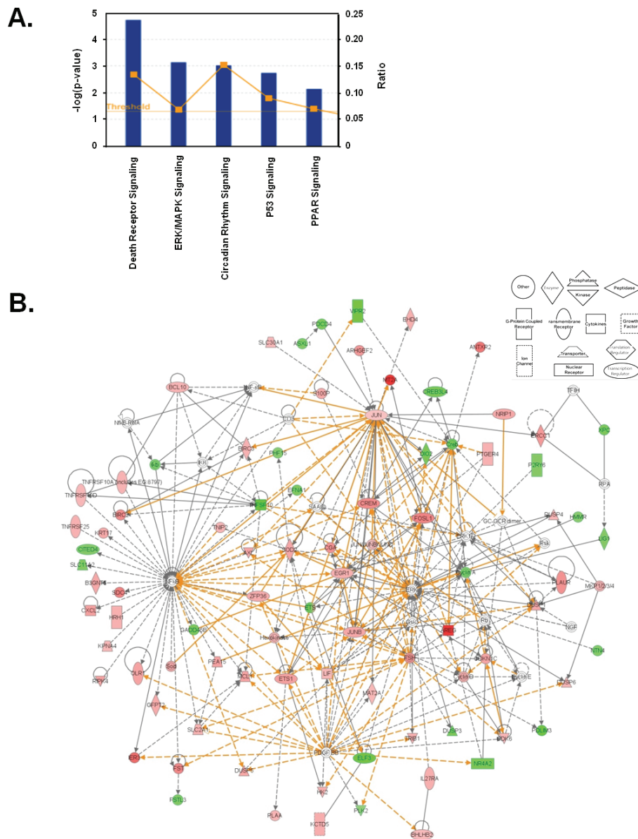
Figure 6 Significant pathways and interactions among EGF-regulated geneset. (A) Core functional analysis of EGF-regulated genes derived from the RankProd test clustering around canonical pathways performed using the Ingenuity Pathway Analysis software. (B) Pathway analysis based on the Ingenuity Pathway Knowledge base. The two best ranked networks holding EGF-regulated genes derived from the RankProd test were merged showing a unique network. Up-regulated genes are indicated in red and down-regulated genes in green. The shape of the node denotes the main function of the protein encoded by the gene (see boxed inset). Continuous lines indicate interaction between the products of the genes; dashed lines indicate an indirect interaction; lines with an arrow indicate that the source gene “acts on” the target gene. Regulated genes are shown as grey boxes and non-regulated but associated with the regulation of some of these genes are shown as white nodes. Orange lines indicate new gene relationships appearing after merging different networks.
