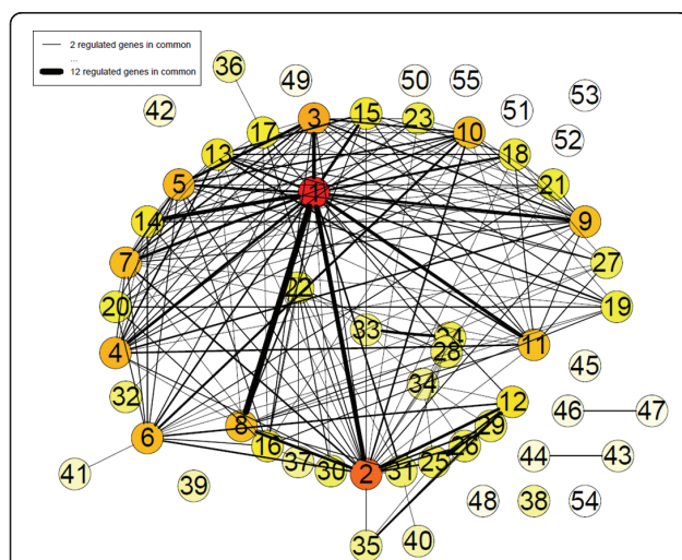
Figure 7 Higher order network of interactions among EGF-regulated genes. Network of genomic interactions among EGF-regulated pathways (Holm-adjusted p-value < 0.01) as defined by GlobalAncova using KEGG database functional annotation. Nodes (pathways) that have at least two regulated genes (as defined by RankProd analysis) in common with other pathways are connected by continuous lines to these other pathways. The strength of each pathway interconnection (i.e. the number of shared regulated genes) is expressed by the width of the continuous lines connecting the two nodes. The node color indicates the interconnectivity of the nodes ranging from no connection to any other pathway (white) to many connections with other pathways (red). Numbers define KEGG categories as listed in Table 3.
