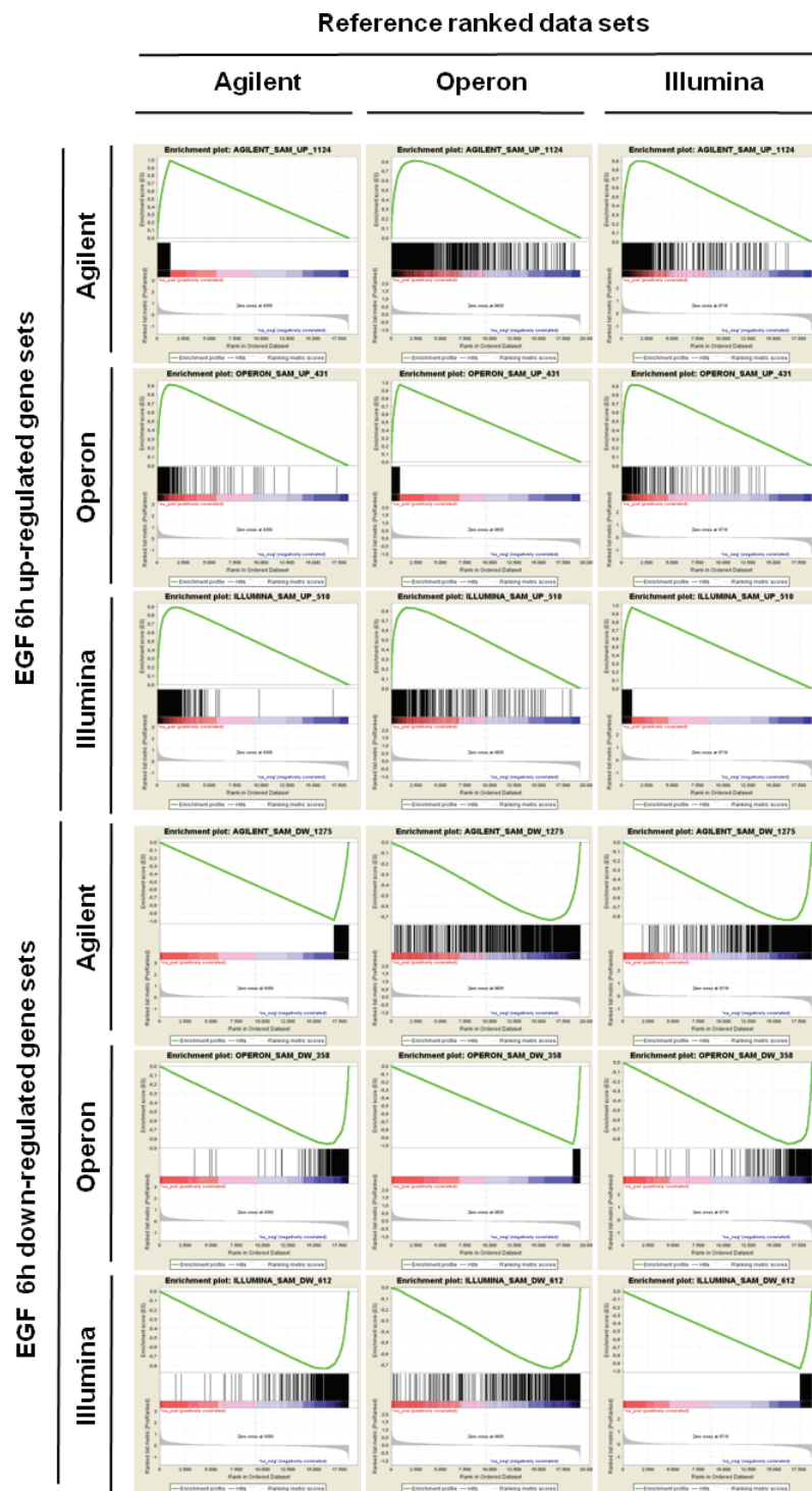
Figure 2 GSEA analysis on significantly regulated gene sets across microarray platforms. Profile of the Running ES Score & Positions of Gene Set Members on the Rank Ordered List using 6 h EGF treatment data according to each of the three microarray platforms. In each panel, the vertical black lines indicate the position of each of the genes of the tested gene set in the reference data (ranked by average of the three respective EGF versus control log2ratios of replicate experiments). The green curve plots the ES (enrichment score), which is the running sum of the weighted enrichment score obtained from GSEA software. Within each queried gene set, the farther the position of a gene to the left (red) implies a higher correlation with EGF up-regulated genes in the reference platform, and the farther to the right (blue) implies a higher correlation with genes down-regulated upon EGF treatment in the reference platform. Studied gene sets correspond to lists of up- or down-regulated genes in each platform at 6 h of EGF treatment. Significantly enriched data sets are defined according to GSEA default settings ( p < 0.001 and a false discovery rate (FDR) < 0.25 ). R.L.M = ranked list metric.
