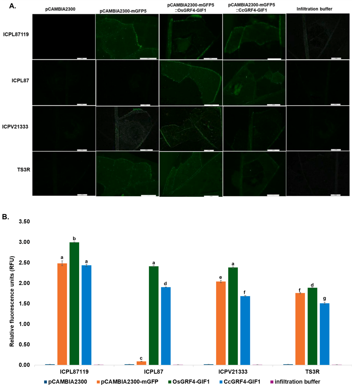
Fig. 3. Quantification of mGFP5 fluorescence in four agroinfiltrated pigeonpea genotypes at 72 h after infiltration using a microplate reader. (A). An overview of mGFP5 fluorescence observed in four pigeonpea genotypes- ICPL87119, ICPL87, ICPV21333, and TS3R. (B) GFP fluorescence quantification was measured at an excitation/emission wavelength of 488/528 nm, and an empty vector and infiltration buffer were used as a reference and negative control, respectively. The fluorescence levels detected in a sample are relative to the levels in reference and infiltration buffer and represented as RFU. The Y-axis represents mean values of normalized fluorescence intensity (RFU), while the X-axis indicates the genotypes. The results are representative of three independent samples, and values indicate the normalized mean \pm standard error of replicates. The mean values followed by the same alphabet on top indicate no difference (Tukey's Test, p < 0.05 ). All the means are statistically significant as determined by one-way ANOVA ( p < 0.05 ). Total four constructs - pCAMBIA2300 (empty vector), pCAMBIA2300-mGFP5, pCAMBIA2300-mGFP5::OsUbi-OsGRF4-GIF1-NosT, pCAMBIA2300-mGFP5::OsUbi-CcGRF4-GIF1-NosT, along with infiltration buffer (negative control) were used for measuring mGFP5 levels.
