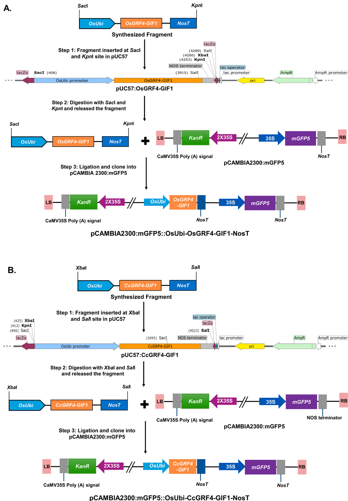
Fig. 1. Schematic diagram showing the cloning of (A) OsUbi-OsGRF4-GIF1-NosT and (B) OsUbi-CcGRF4-GIF1-NosT into pCAMBIA2300-mGFP5 binary vector.
