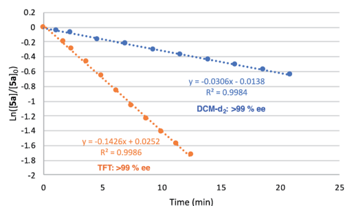
Fig. 9 Plot of \ln([5a]/[5a]_0) vs. time of model substrate 5a to pyrrolidine 5b vs. time (min) using ( R a ,R a ,S,S )-2[NTf 2 ] at 0.5 mol%. Reactions conducted in DCM-d 2 or TFT (0.5 mL), [5a] = 0.6 M, [Ir] = 0.003 M. Conversion monitored using 1 H NMR.
