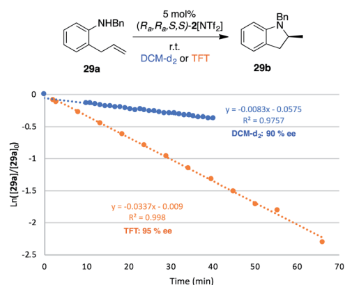
Fig. 10 Plot of Ln([29a] t /[29a] 0 ) vs. time of substrate 29a to indoline 29b using ( R a ,R a ,S,S )-2[NTf 2 ] at 5 mol%. Reactions conducted in DCM-d 2 or TFT (0.5 mL), [29a] = 0.6 M, [Ir] = 0.03 M. Conversion monitored using 1 H NMR.
