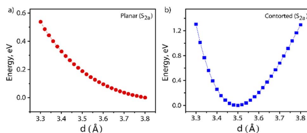
Fig. 5 Potential energy surface plot for the geometry scan of the first excited singlet state ( S_{2a} ) of: (a) planar and (b) contorted PPD . The centre-to-centre distance ( d ) of 3.50 Å shows the minima for the contorted PPD .
