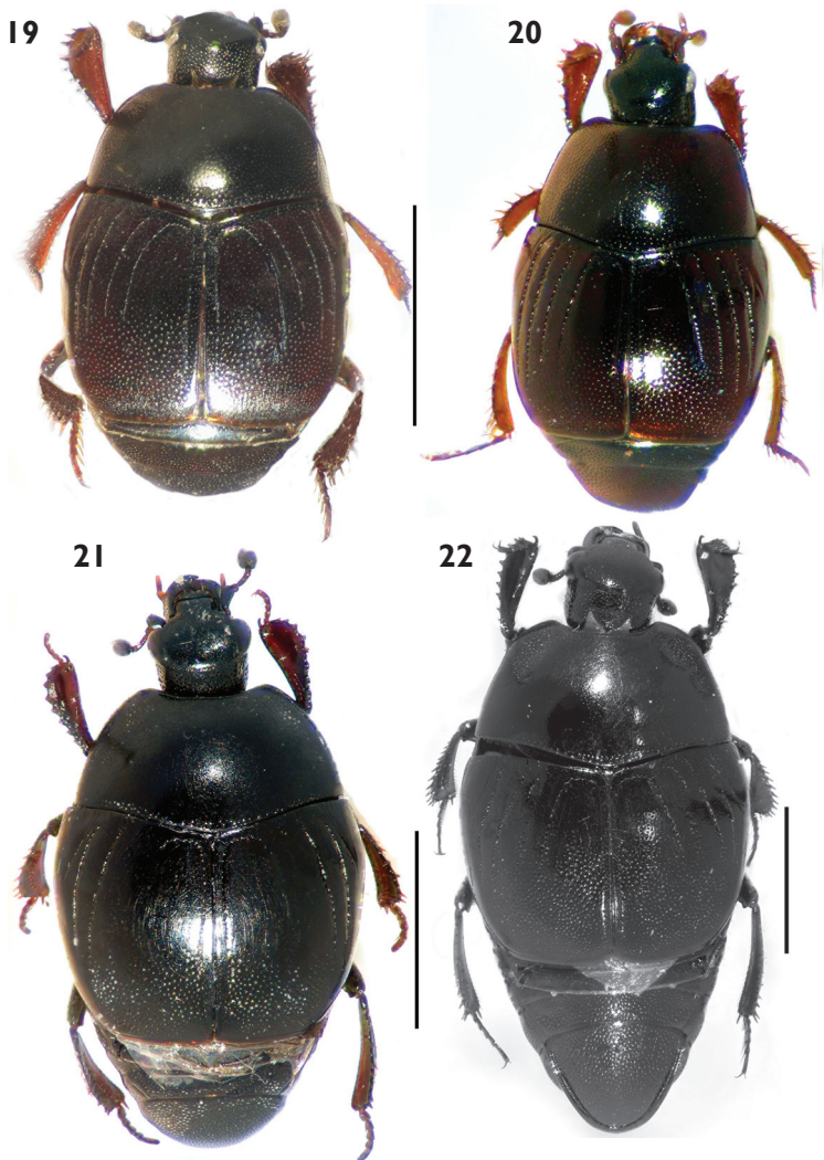
Figures 19–22. Habitus in dorsal view. 19 Euspilotus (Hesperosaprinus) modestus 20 Euspilotus (Hesperosaprinus) parenthesis 21 Euspilotus (Hesperosaprinus) connectens 22 Euspilotus (Hesperosaprinus) azureus . Scale bars: 2 mm.
