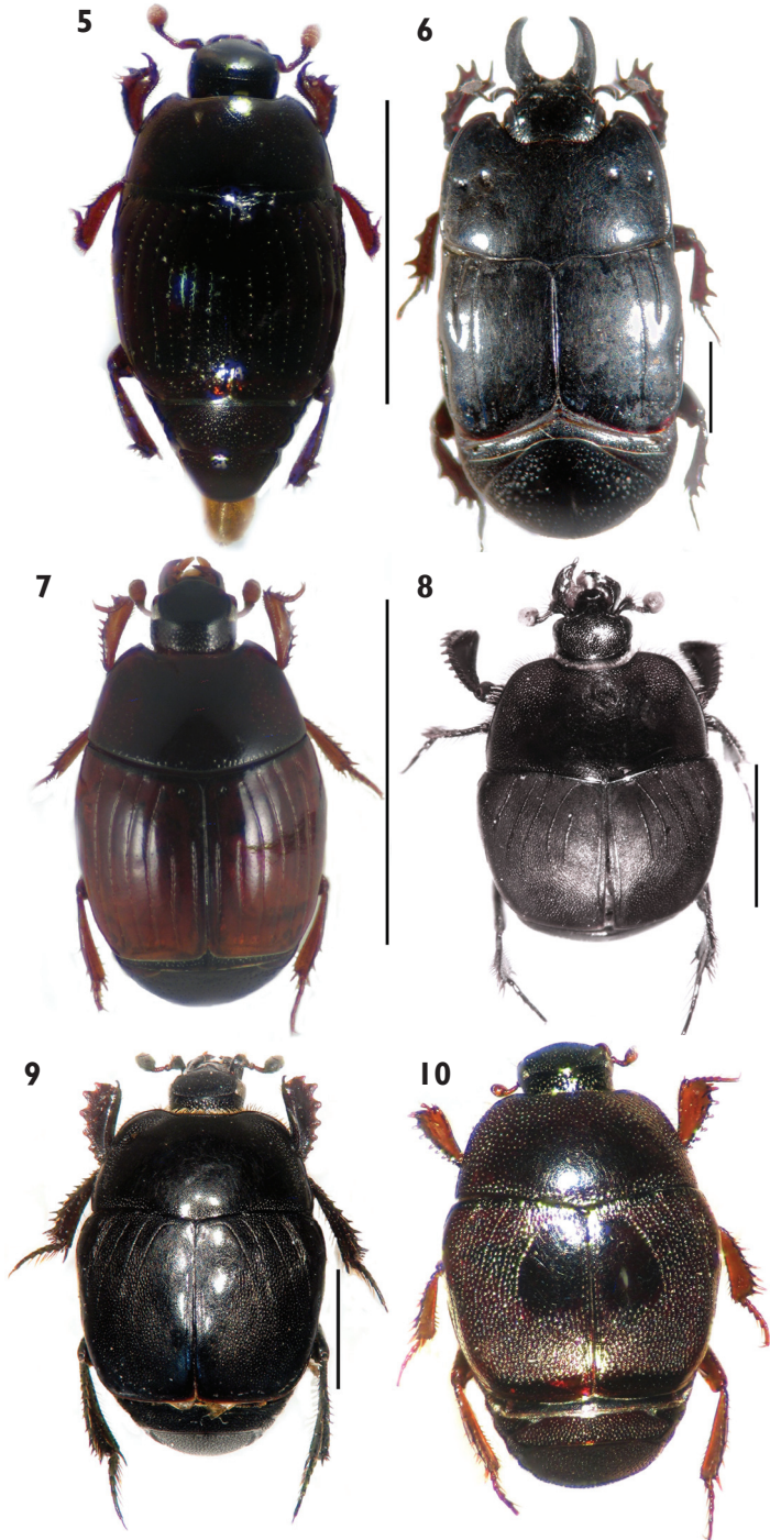
Figures 5–10. Habitus in dorsal view. 5 Carcinops ( Carcinops ) troglodytes 6 Hololepta ( Leionota ) reichii . 7 Pbelister rufinotus 8 Euspilotus (s. str.) lacordairei 9 Euspilotus (s. str.) patagonicus 10 Xerosaprinus ( Xerosaprinus ) diptychus . Scale bars: 2 mm. Scale bars: 2 mm.
