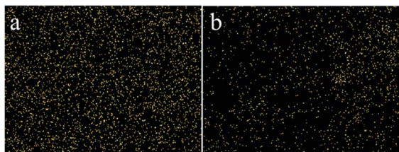
Fig. 6 The EDX maps of the Cr content on the adsorbents after adsorption. (a) IIZMS-APTRES, and (b) NIZMS-APTRES.
