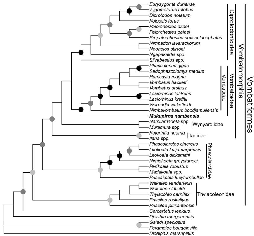
Figure 5. Phylogeny of Vombatiformes based on undated Bayesian analysis of a morphological dataset comprising 79 craniodental characters scored for 36 fossil and extant vombatiforms and five non-vombatiform outgroup taxa. The analysis used the Mk v model as implemented in MrBayes 3.2.7, with rate heterogeneity between characters modelled using an eight category lognormal distribution. The topology is a majority rule consensus of post-burn-in trees, retaining compatible partitions with Bayesian posterior probability (BPP) < 0.5. Black circles at nodes represent Bayesian posterior probability (BPP) of \geq 0.95 , dark grey circles represent BPP of 0.75–0.94 and light grey circles represent BPP of 0.5–0.74. Nodes without circles have BPP < 0.5. Mukupirna nambensis is shown in bold.
