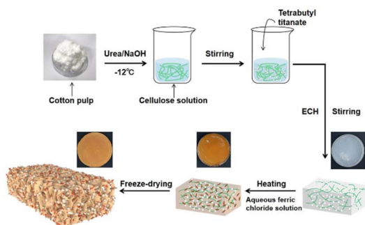
Fig. 1 Schematic diagram for preparation process of \beta -FeOOH/TiO 2 /cellulose nanocomposite aerogel.
