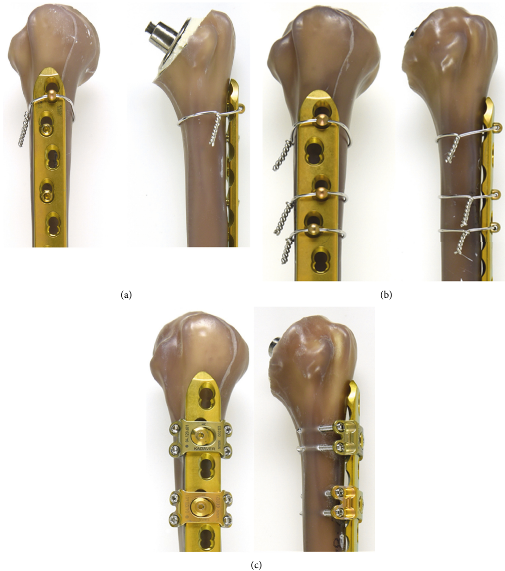
FIGURE 1: (a). LCP plate fixed on the humerus using 1 × 1.5 mm cerclage wires placed at the level of the 1 st hole and 2x unicortical locking screws placed at the levels of the 3 rd and 4 th holes. (b) LCP plate fixed on the humerus using 3 × 1.5 mm cerclage wires placed at the levels of the 1 st , 3 rd , and 4 th holes. (c) LCP plate fixed on the humerus using 2x locking attachment plates allowing bicortical fixation placed at the levels of the 2 nd and 4 th holes.
