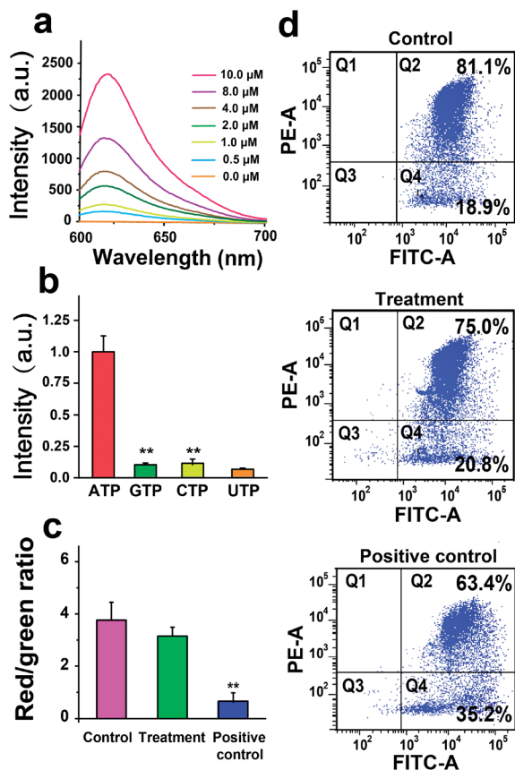
Fig. 2 Characterization of the AMP. (a) The fluorescence intensity of the AMP ( 1 \mu\text{M} ) with increasing the ATP concentration from 0 to 10 \mu\text{M} . (b) The fluorescence intensity of the AMP ( 1 \mu\text{M} ) treated with 1 \mu\text{M} ATP, GTP, UTP, or CTP. (c) The JC-1 red/green fluorescence ratio showing the mitochondrial membrane potential (MMP) of U251 cells. Control: U251 cells in PBS; treatment: U251 cells treated with the AMP ( 1 \mu\text{M} ); positive control: U251 cells treated with carbonyl cyanide m -chlorophenylhydrazone (CCCP, a mitochondrial uncoupler, 10 \mu\text{M} ). (d) Flow cytometry measuring the red aggregate and green monomeric fluorescence of JC-1 in U251 cells under different treatments. **P < 0.01 , n = 3 , t -test.
