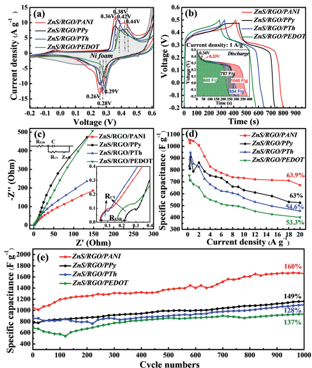
Fig. 2 In three-electrode system, (a) CV curves at 10 mV s -1 , (b) GCD profiles and discharge curves (illustration) at 1 A g -1 , (c) high frequency (illustration) and low frequency Nyquist plots at frequency range from 100 kHz to 0.01 Hz, (d) capacitance performance at the range of current density from 0.3 to 20 A g -1 and (e) cycle performance of ZnS/RGO/PANI, ZnS/RGO/PPy, ZnS/RGO/PTh and ZnS/RGO/PEDOT.
