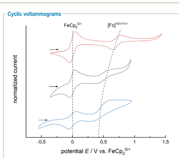
Fig. 2 Cyclic voltammograms of compounds \text{FeC}_{10}(\text{HgO}_2\text{CCF}_3)_{10} in THF with 0.1\text{ M TBAPF}_6 as supporting electrolyte (bottom), 26 [\text{FeC}_{10}(\text{HgTHT})_{10}][\text{SbF}_6]_{10} ( 2b , middle) and [\text{FeC}_{10}(\text{HgMeCN})_{10}][\text{SbF}_6]_{10} ( 2c , top) in acetonitrile without supporting electrolyte at 100\text{ mV s}^{-1} scan rate and room temperature.
